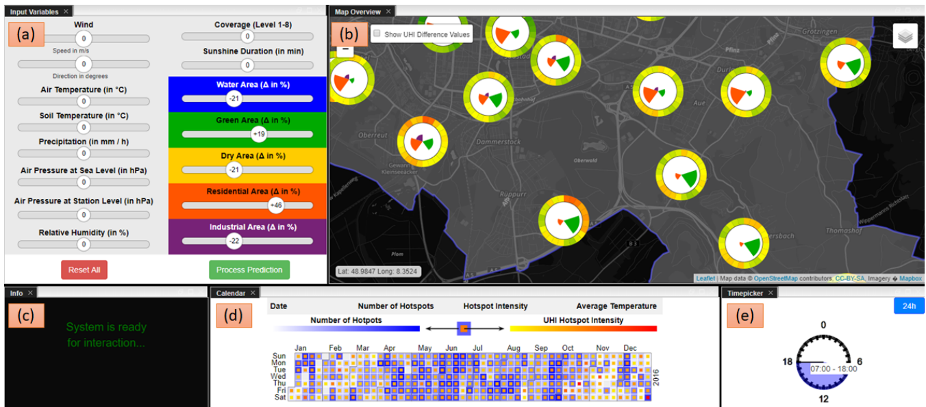
Figure 3: Our system consists of five components that can be flexibly resized by the user: the Feature Input Panel (a) allows to predict the influence of 15 environmental parameters on the UHI event outcome. The colors correspond to the Nightingale glyph in (b). The Nightingale glyph map (b) visualizes the temporal occurrence of UHI events and the surrounding spatial context of stations in Karlsruhe. The system status panel (c) displays information feedback about the system’s state to the user. The interactive calendar view (d) depicts the number of hotspot and their intensity for each day over an entire year. Users can select time ranges to filter the Nightingale glyphs in (b). The time selector (e) enables users to apply an hourly-based filter to both the Nightingale glyph map (b) and the calendar view (d) using the clock metaphor.
