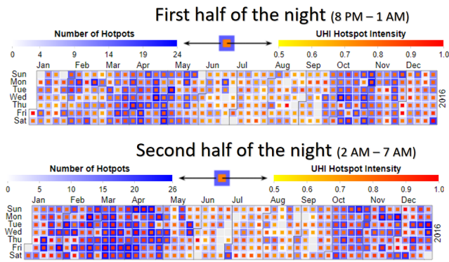
Figure 10: Comparison of UHI hotspots characteristics for the first and second half of the night.
