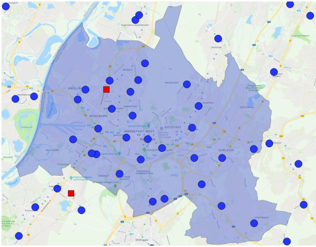
Figure 2: Distribution of private weather stations (blue circles) and stations from the DWD (red squares) in and around the city of Karlsruhe. The volunteered data set provides a more fine-grained spatial distribution: 28 stations in the city of Karlsruhe.
