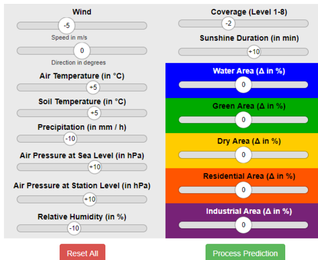
Figure 8: Adjusted feature parameters to simulate a warmer and drier weather situation.
