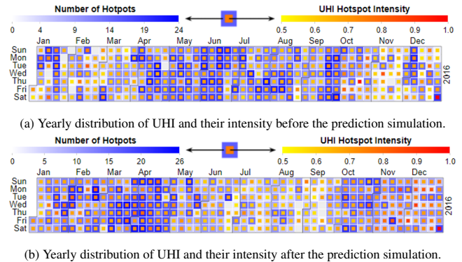
Figure 9: Overview of the emergence of urban heat islands and their average intensity per day for a year before and after executing a warm weather simulation.
